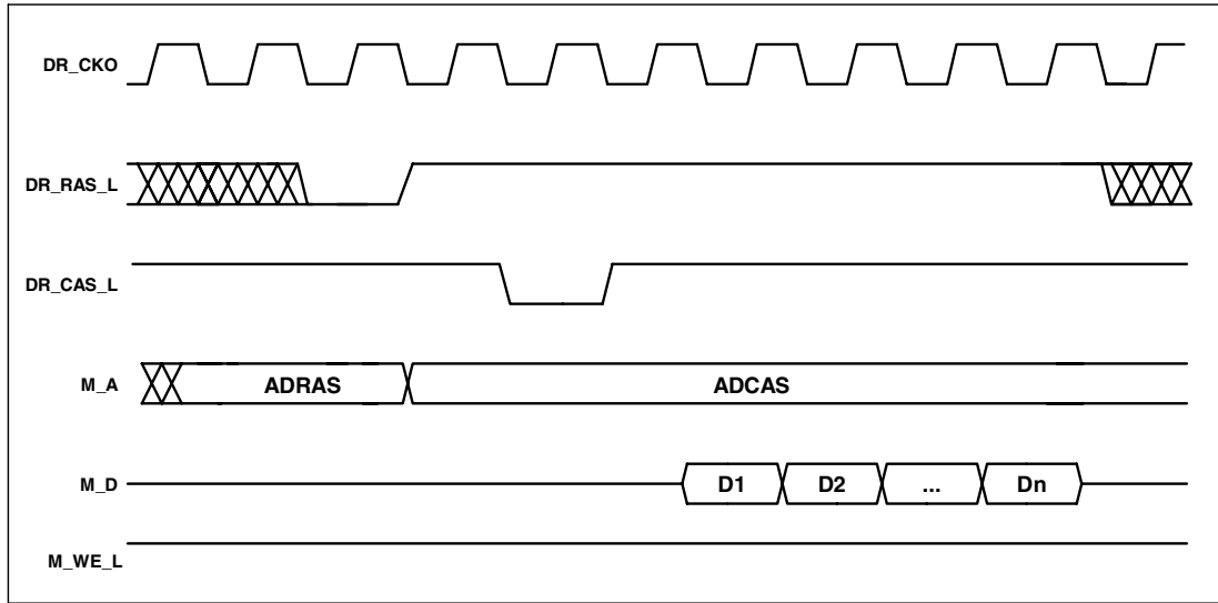
Figure 4. SDRAM Burst Read
