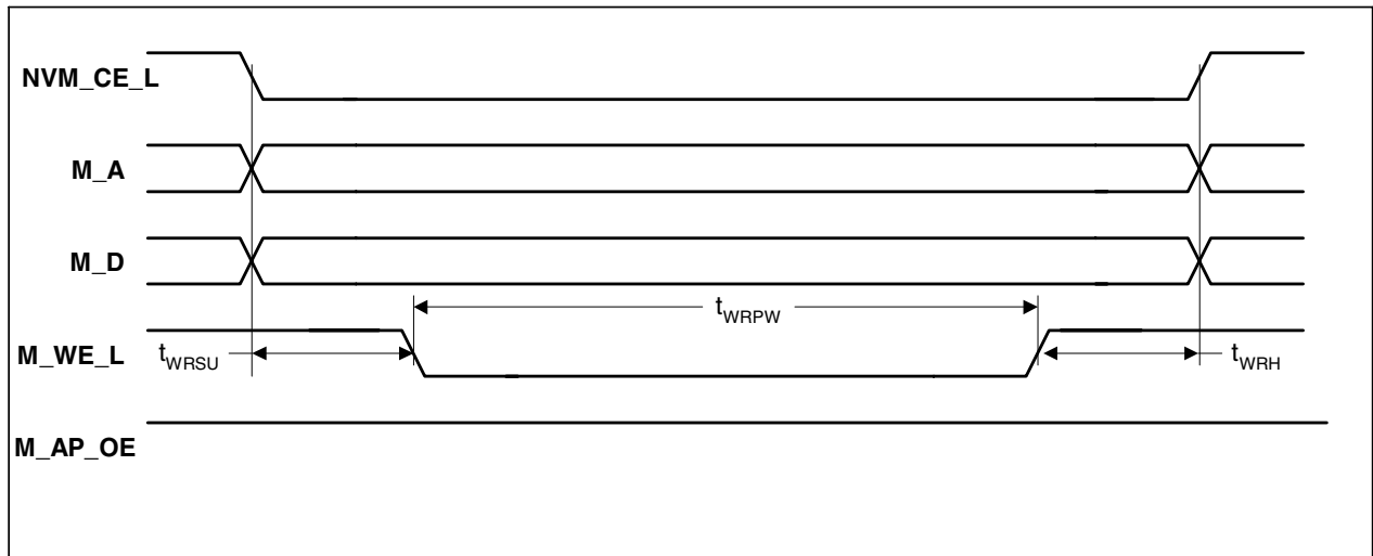
Figure 11. FLASH/ROM Write
